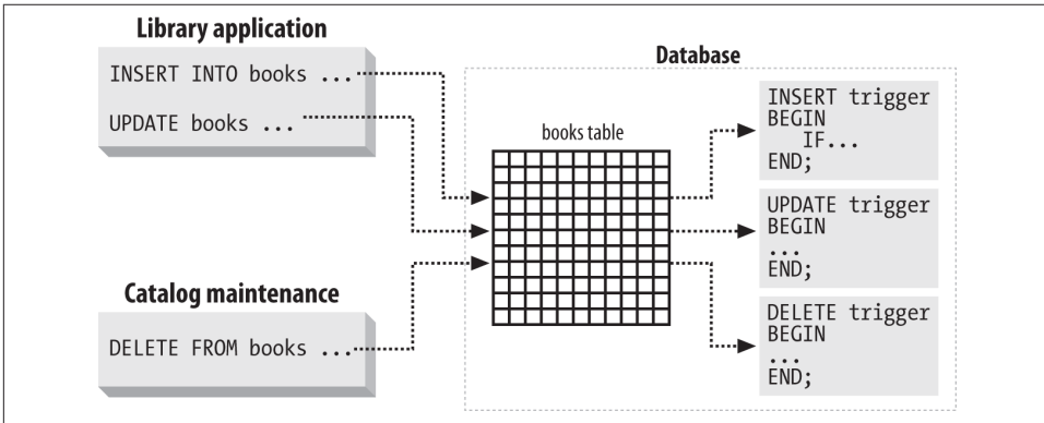
Figure 19-1. DML trigger flow of control
