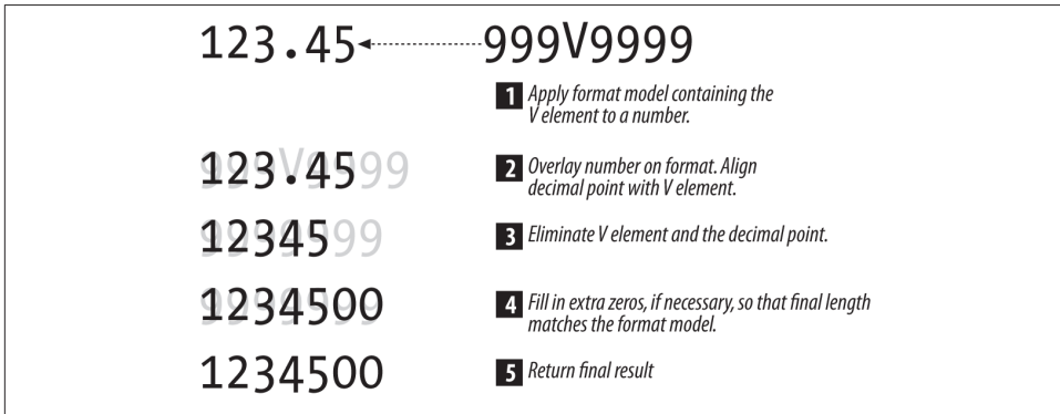
Figure 9-4. The V number format element
