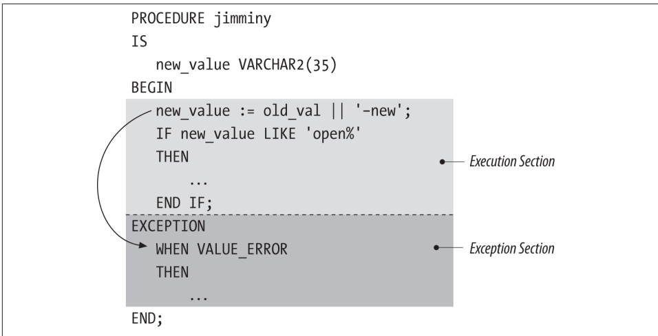
Figure 6-1. Exception-handling architecture
