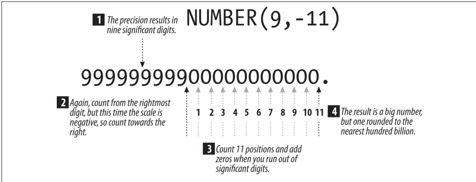
Figure 9-3. The effect of negative scale
