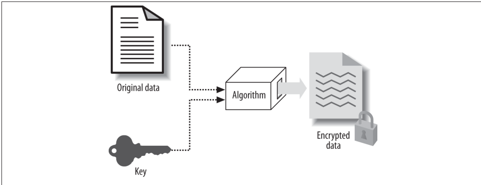
Figure 23-1. Encryption basics
